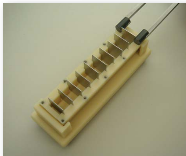
Lifter Block for loading and unloading of cassette with edge grip mechanical tools
